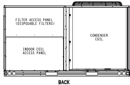
BACK
