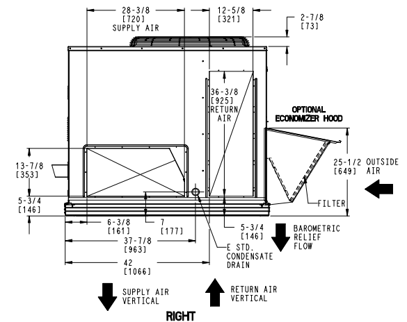
RIGHT
